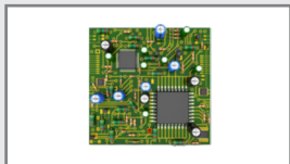
Item: POE1 Power Over Ethernet board: - dual POE++ input on eth 2/4 - POE output on eth 1 (external Wifi, Bluetooth antenna)
